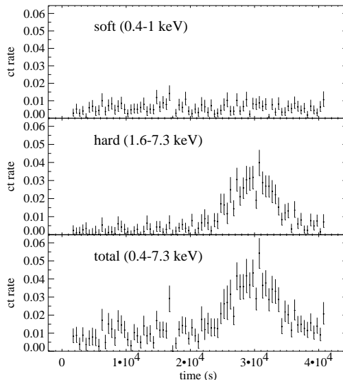
Fig. 13.— X-ray light curves of DG Tau A. The top panel shows the soft component, the middle panel the hard component, and the bottom the total X-ray light curve. (Güdel et al. , 2006b, in preparation.)
