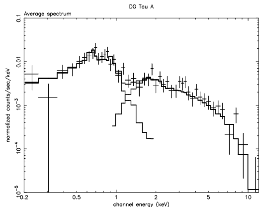
Fig. 12.— Average spectrum of DG Tau A. Also shown is the fit to the spectrum (black histogram) and its two constituents, the soft and the hard components. (Güdel et al. , 2006b, in preparation.)
