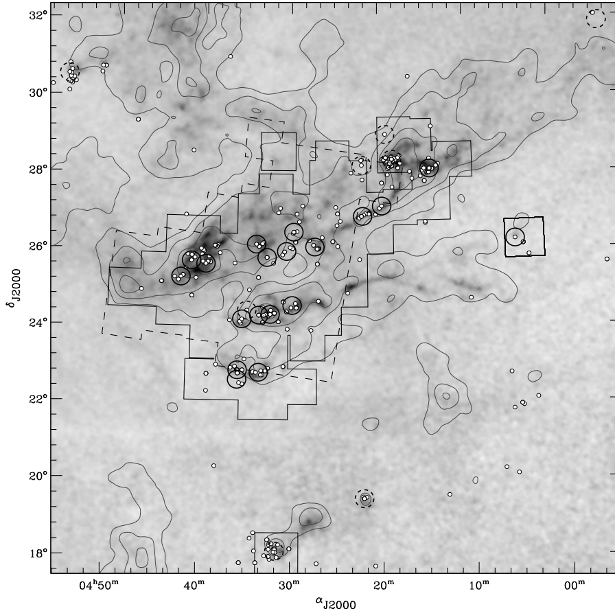
Fig. 1.— Map of the TMC region. The grayscale background map is an extinction ( A_V ) map from Dobashi et al. (2005) . The outlines of the CFHT and the Spitzer surveys are indicated by the solid and dashed polygons, respectively. The large (0.5 degrees diameter) circles show the fields of view of the XMM-Newton X-ray survey (the dashed circles marking fields from separate projects also used for the survey). Small white dots mark the positions of individual young stars. Note the outlying XMM-Newton fields around SU Aur (NE corner), \zeta Per (NW corner), and L1551 and T Tau (south). (Figure courtesy of Nicolas Grosso.)
