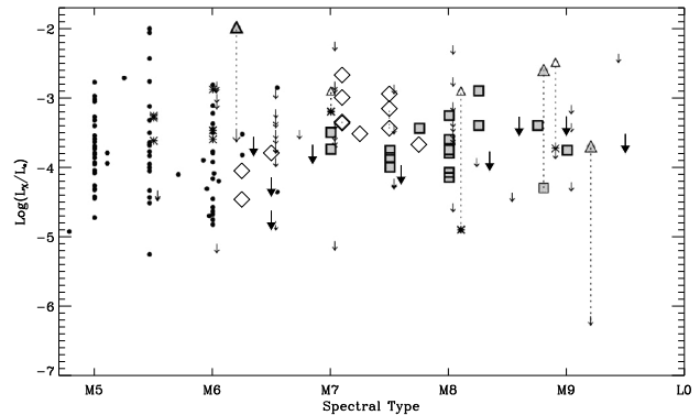
Fig. 5.— L_X/L_* of low-mass stars and BDs as a function of spectral class, including samples of late-type main-sequence field stars (asterisks, Fleming et al. , 1993), the Orion Nebula Cluster BD sample (filled squares, triangles, and small arrows) and T Tauri stars later than M5 (filled dots) from Preibisch et al. (2005b), and our sample of TMC detections (diamonds) and upper limits (arrows). (Figure courtesy of Nicolas Grosso.)
