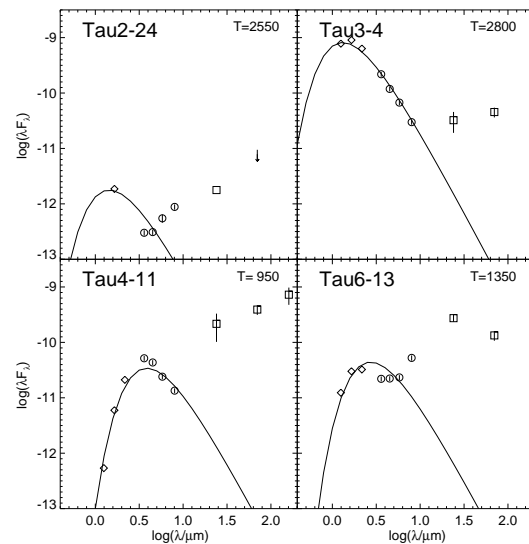
Fig. 3.— 2MASS NIR + Spitzer IRAC and MIPS spectral energy distributions of four bright 24 \mu\text{m} sources discovered in the course of the survey. Temperatures indicated in the plots are effective temperatures of the plotted photosphere.
