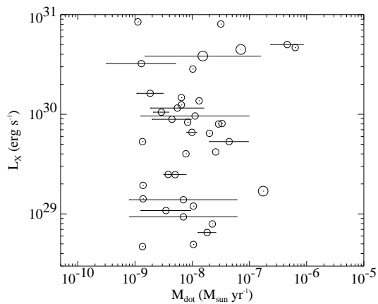
Fig. 11.— Scatter plot of L_X versus the (range of) mass accretion rates reported in the literature. No trend is evident. Symbols are as in Fig. 7. (Telleschi et al. 2006, in preparation.)
