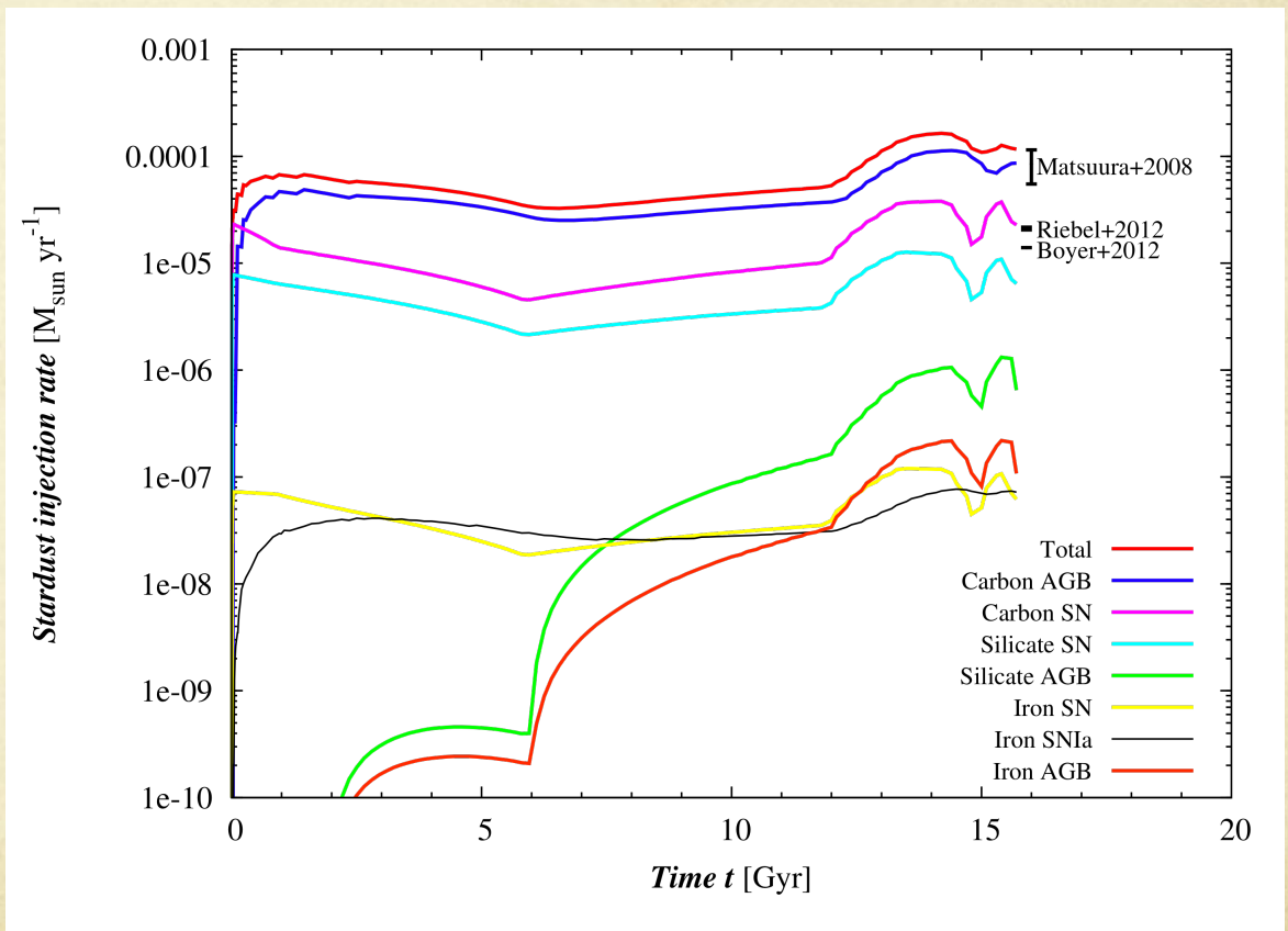
Global stardust production rates during LMC evolution
