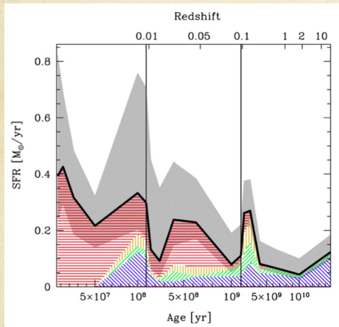
Input SFH for chemical evolution model
