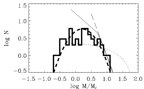
Fig. 3.— The IMF that results from isothermal gravitational fragmentation (e.g., Fig. 2) is typically broad and log-normal in shape (Klessen et al. , 1998). The stellar masses are measured in terms of the average initial Jeans mass of the cloud.
