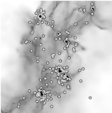
Fig. 10.— The location of the massive stars (dark circles) is shown to be in the centre of individual subclusters of low-mass stars (light circles) due to competitive accretion (cf. Bonnell et al., 2004 ).
