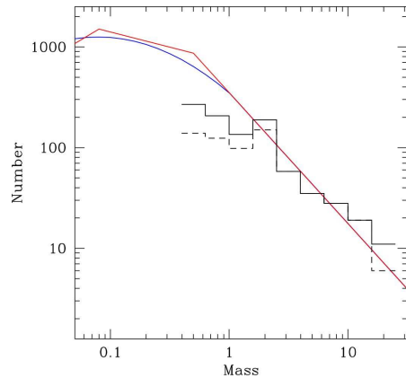
Fig. 1.— The IMF for NGC3603 (Stolte et al., 2006) is shown as a histogram in log mass ( dN(\log \text{mass}) ) for the completeness corrected (solid) and uncorrected (dashed) populations. For comparison, the Kroupa (2001) segmented power-law and the Chabrier (2003) log-normal plus power-law IMFs are also plotted in terms of log mass.
