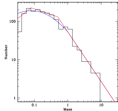
Fig. 9.— The resulting IMF from a simulation of the fragmentation and competitive accretion in a forming stellar cluster (e.g., Bonnell et al., 2003) is shown as a function of log mass ( dN(\log \text{mass}) ). Overplotted is the three segment power-law IMF from Kroupa (2001) and Chabrier’s (2003) log-normal plus power-law IMF. The masses from the simulation have been rescaled to reflect an initial Jeans mass of \approx 0.5 M_{\odot} .
